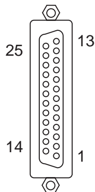
Pin Out DVB SPI Interface
